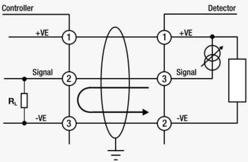
XCD Source Configuration
