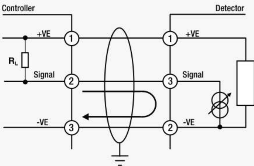
XCD Sink Configuration
