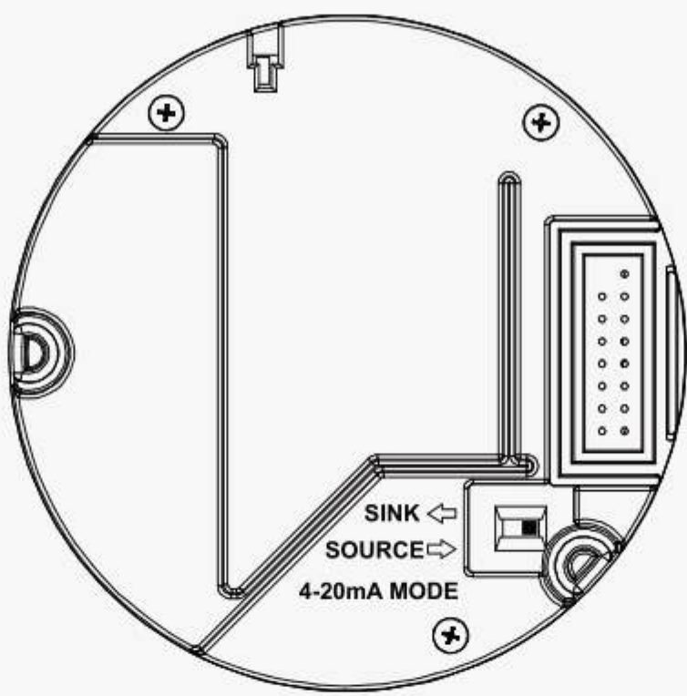
Puck Rear View
